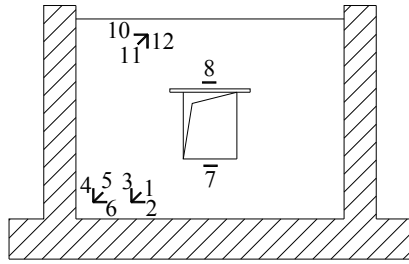
Fig. 4 Distribution of Strain rosettes
