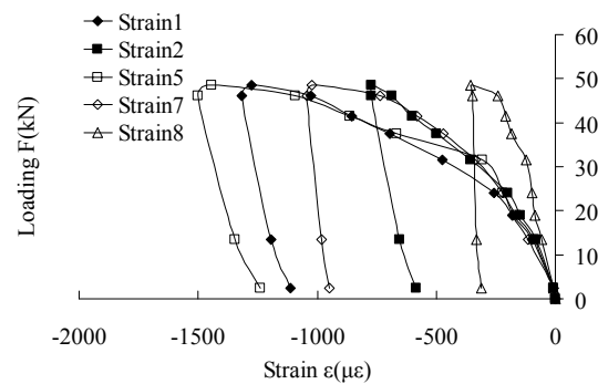
Fig. 9 Loading-Strain Curve of W2
