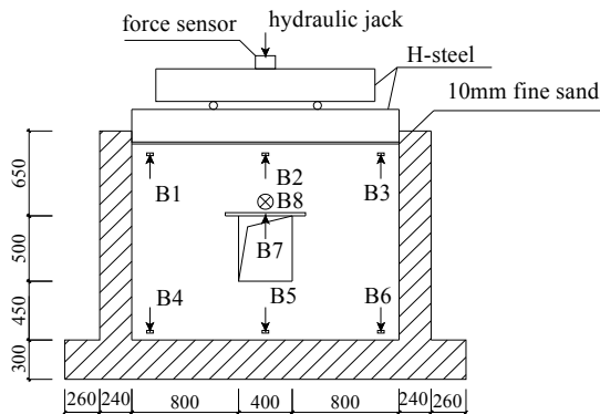
Fig. 2 Loading system (B refers to dial gauge)
