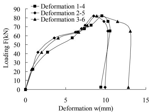
Fig. 8 Loading-Deformation Curve of W3
